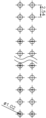
Recommended P.C.Board Hole Layout
