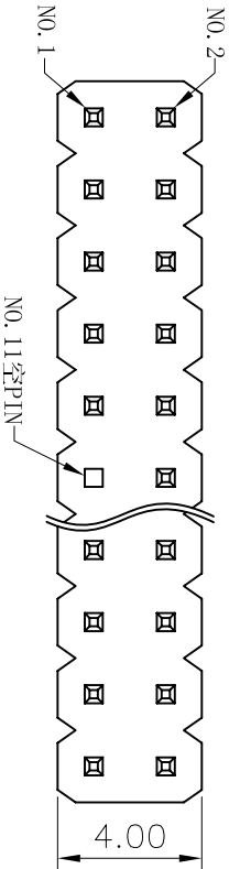
Recommended P.C.Board Hole Layout
