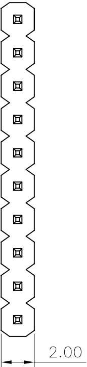
Recommended P.C.Board Hole Layout
