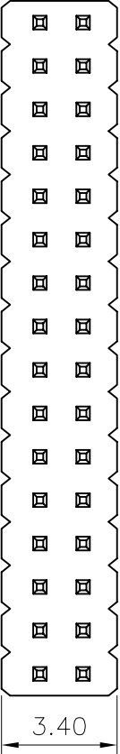
Recommended P.C.Board Hole Layout (Tolerance:±0.05)
