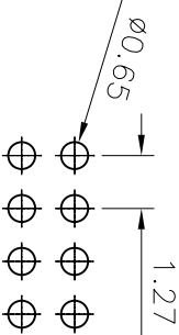
Recommended P.C.Board Hole Layout (Tolerance:±0.05)
