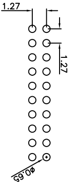
Recommended P.C.Board Hole Layout
